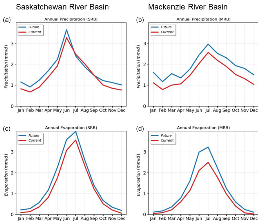
Figure 2. Simulated P and ET surface water budget components ( \text{mm d}^{-1} ) over the Saskatchewan (a, c) and Mackenzie (b, d) River Basins for the WRF control (current; 2000–2015) and future (2085–2100) periods. Results are from Kurkute et al. (2020).
