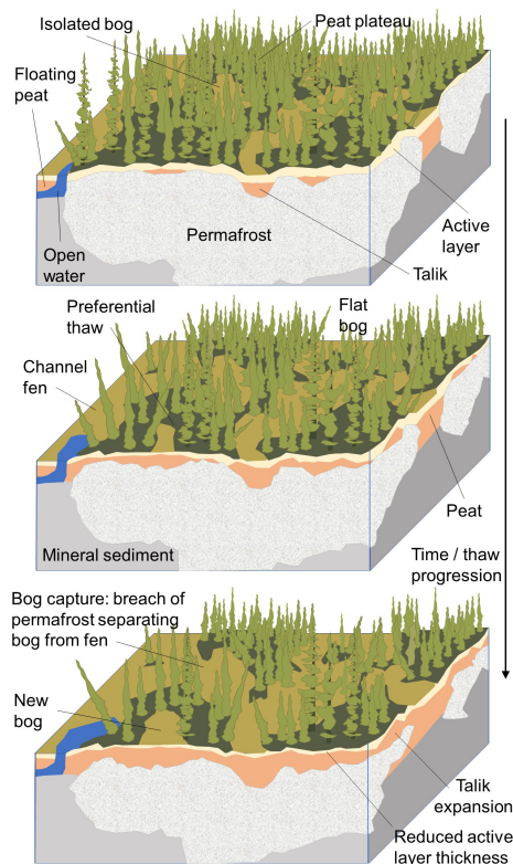
Figure 8. Conceptual model of forest canopy thinning and permafrost thaw in the Taiga Plain, after Quinton et al. (2009, 2019) and Connon et al. (2018).
