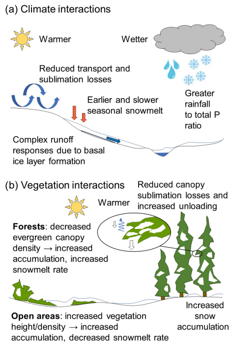
Figure 4. Conceptual schematic of expected snow change in the CCRN domain and similar cold regions. Warmer conditions lead to less snow, while wetter conditions can lead to more or less snow; warmer and wetter conditions can be partially compensatory. Other changes complicate the snow–climate interactions, and spatial patterns of vegetation change with respect to snow processes control snow response.
