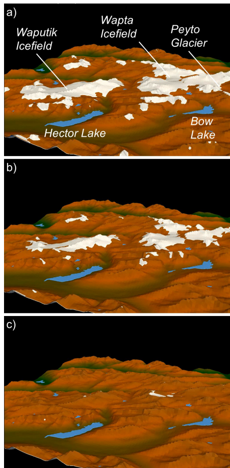
Figure 5. Simulated glacier projections in 3D perspective along the continental divide and in the headwaters of the Saskatchewan River for (a) 2005, (b) 2040, and (c) 2085 using the Canadian Earth System Model under the RCP8.5 forcing scenario. Scale varies in the perspective, but the ground distance across the length of the Waputik Icefield in the 2005 scene is roughly 12 km. Results are from Clarke et al. (2015).
