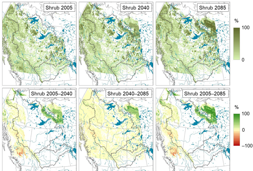
Figure 7. Changing shrub cover fractions over the Mackenzie and Saskatchewan River Basins in the 21st century derived from CCRN expert-guided modifications to climate-based projections using the methodology of Rehfeldt et al. (2012) (Appendix). Projections were made in 45-year increments from the base period (centered at 1995 but using the 2005 base map) to represent the 2040 (mid-century) and 2085 (late-century) periods.
