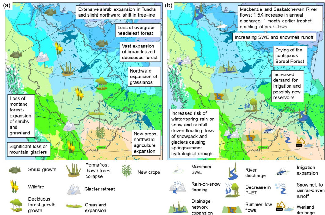
Figure 9. Conceptual depiction and synthesis of surface changes over the CCRN region, by the late 21st century, for (a) land cover and vegetation and (b) hydrological regime and water management. The base map depicts the Level II Ecological Regions of North America as shown in Fig. 1.
