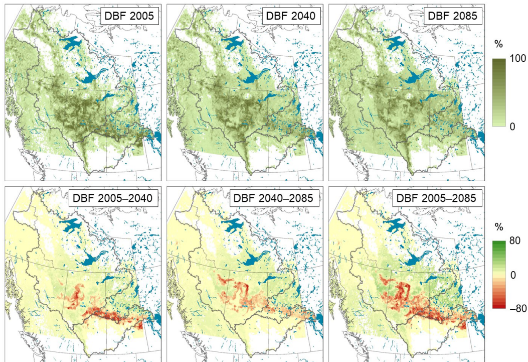
Figure 6. Changing DBF cover fractions over the Mackenzie and Saskatchewan River Basins in the 21st century. The approach involved a simple yet ecologically based projection with expert-guided modifications to impose restrictions on the rates of species colonization and requirements for wildfire to trigger change (Appendix). Projections were made in 45-year increments from the base period (centered at 1995 but using the 2005 base map) to represent the 2040 (mid-century) and 2085 (late-century) periods.
