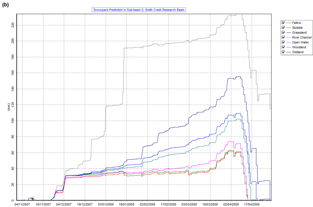
Figure 29. Simulation of snow accumulation development for Smith Creek Research Basin during 31 October 2007-30 April 2008: (a) sub-basin 1 (b) sub-basin 2 (c) sub-basin 3 (d) sub-basin 4 (e) sub-basin 5.
