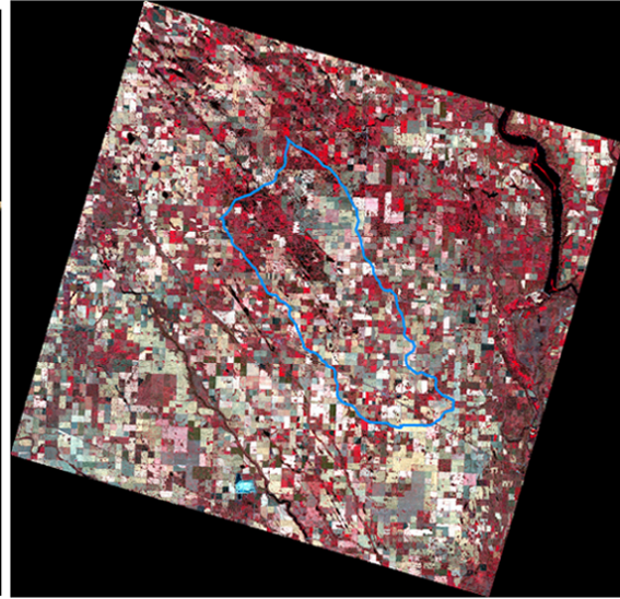
Figure 15. SPOT 5 10-m multispectral images. (a) 2007 summer image and (b) 2008 fall image.
