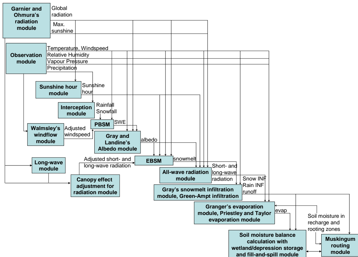
Figure 16. Flowchart of physically based hydrological modules for PHM.
