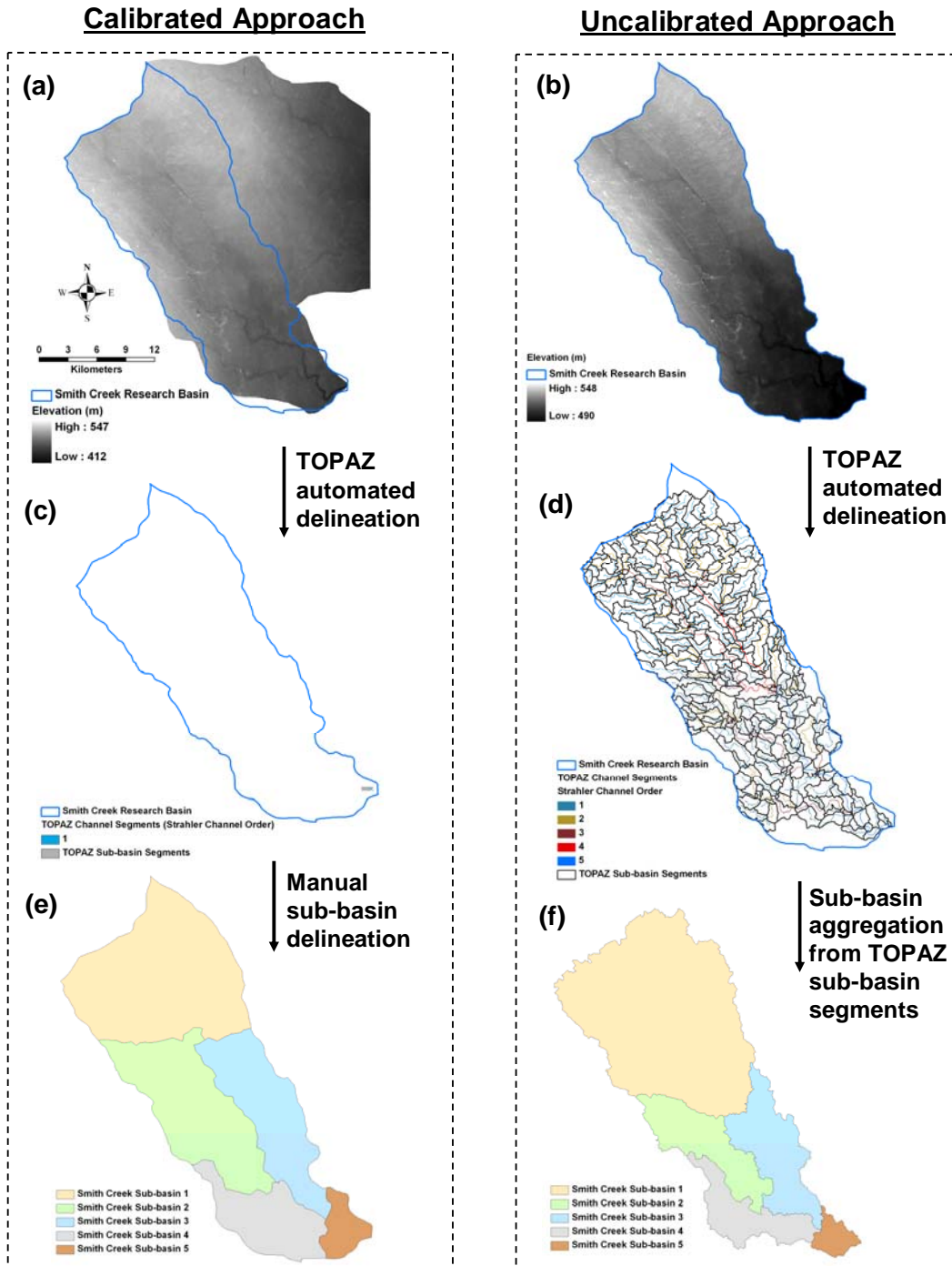
Figure 21. Pre-processing procedure for deriving sub-basins at Smith Creek Research Basin. (a) 50-m resampled topographic map based DEM, (b) 50-m resampled LiDAR DEM, (c) TOPAZ channel and sub-basin segments from the calibrated non-LiDAR approach, (d) TOPAZ channel and sub-basin segments from the Uncalibrated LiDAR approach, (e) sub-basins from the calibrated non-LiDAR approach, and (f) sub-basins from the uncalibrated LiDAR approach.
