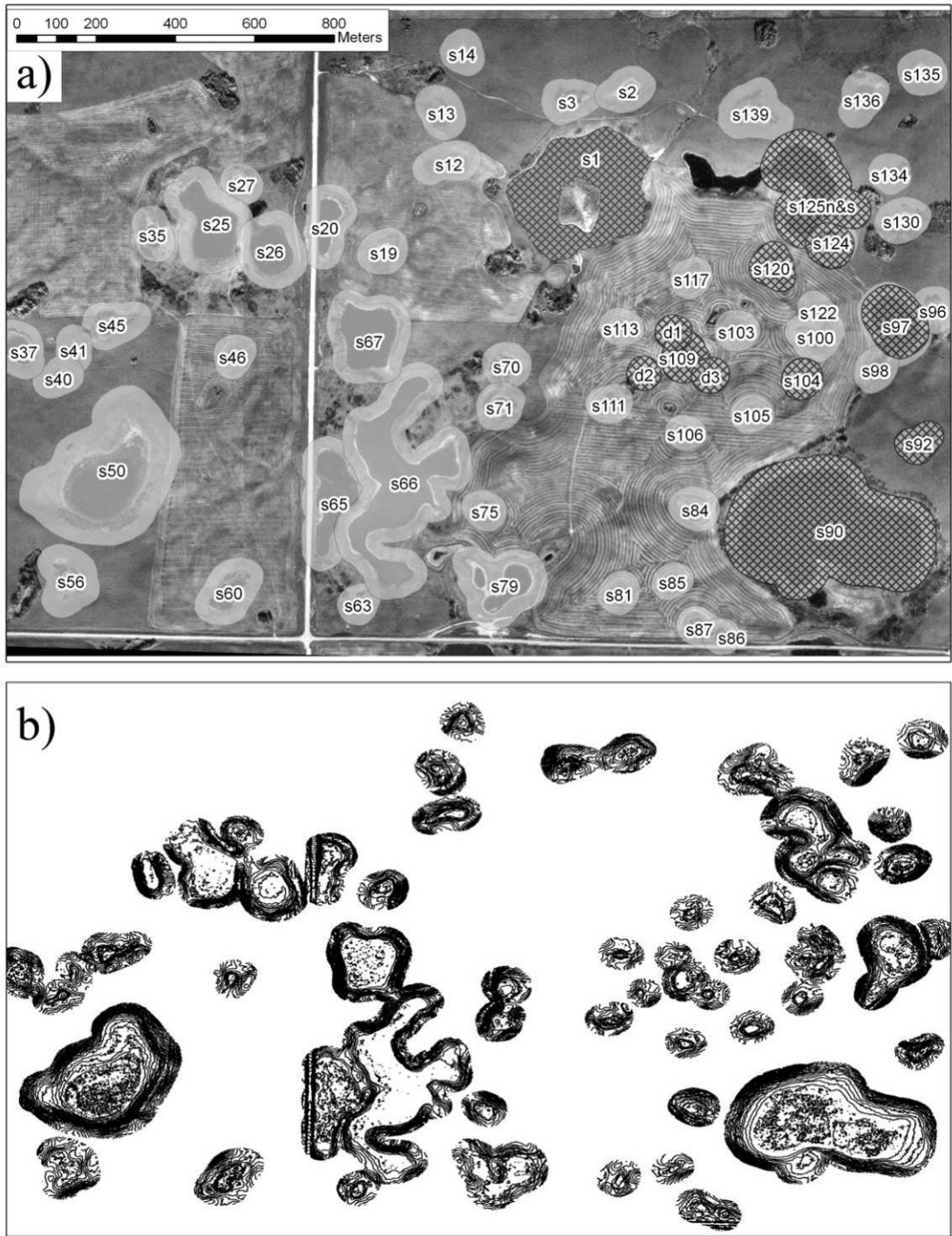
Figure 28. SDNWA study site. (a) air photo (1997) with wetlands delineated and buffered, wetlands with actual volumes indicated by cross-hatching and (b) elevation contours derived from LiDAR DEM.
