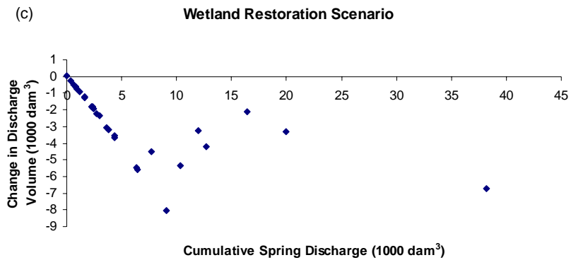
Figure 48. Sensitivity of the Smith Creek cumulative spring discharge during 1965-82 and 1993-2005 periods: (a) forest conversion scenario, (b) agricultural conversion scenario, (c) wetland restoration scenario, and (d) wetland drainage scenario.
