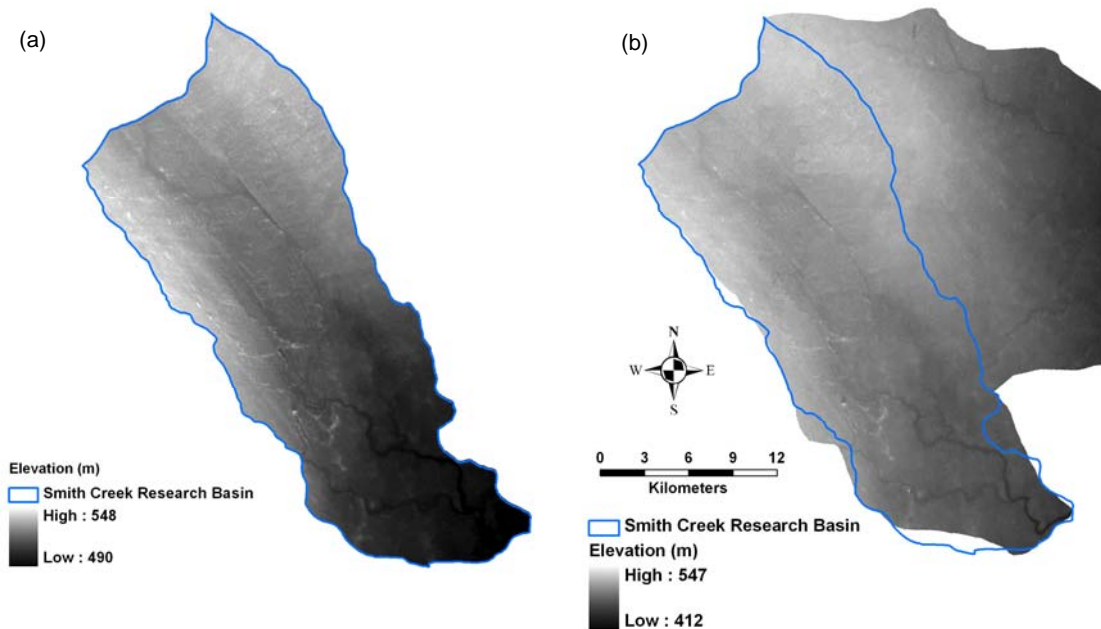
Figure 14. DEMs (a) 1-m LiDAR derived DEM and (b) 25-m topographic map based DEM.
