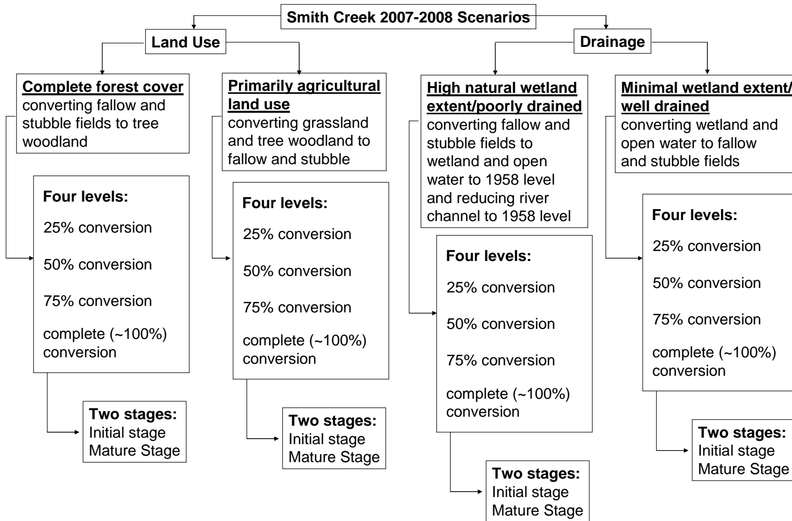
Figure 39. Development of Smith Creek 2007-2008 scenarios.
