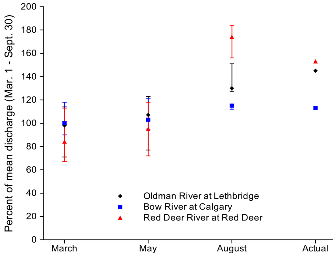
Figure 42. Alberta Environment and Water water supply forecasts for March through September 2011, made in March, May, and August and 2011 actual streamflow volume compared to long-term mean streamflow volumes. The error bars denote the maximum and minimum values of the forecast cumulative flows.
