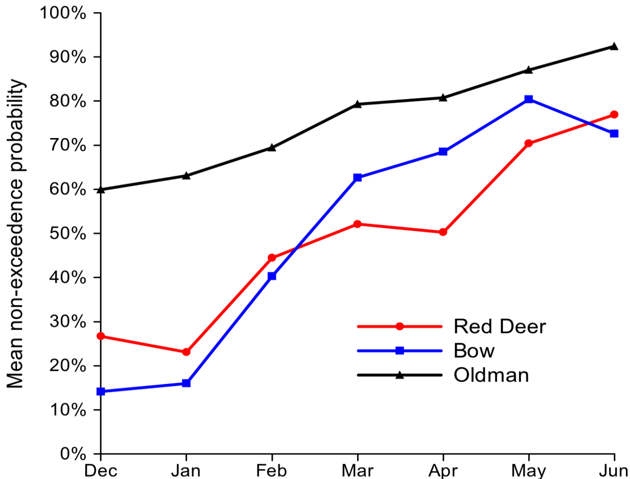
Figure 20. Mean non-exceedence probabilities of the snow surveys in the headwaters of the Oldman, Bow and Red Deer Rivers. Mean values were computed for each month by basin by simple averaging. All data were obtained from the Alberta Environment web site http://www.environment.alberta.ca/forecasting/WaterSupply/index.html .
