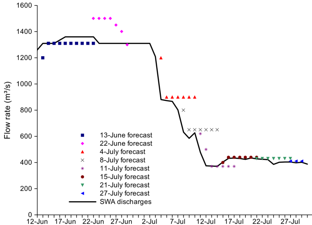
Figure 47. Short-term forecasts of discharges from Lake Diefenbaker and discharges (sum of spillway and powerhouse flows) computed by SWA.
