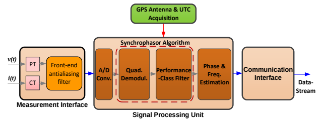
Fig. 3. Typical elements of a phasor measurement unit (PMU).
