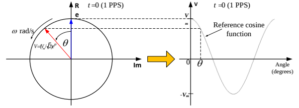
Fig. 2. Synchrophasor representation of a signal v(t) .
