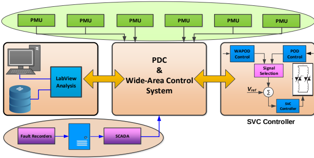
Fig. 6. Architecture of the Statnett power oscillation monitoring and damping system [105].
