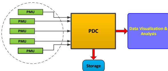
Fig. 4. Architecture of a phasor data concentrator.
