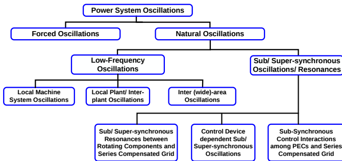
Fig. 5. Classification of power system oscillations.
