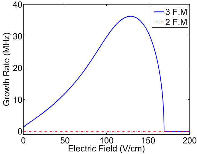
FIG. 10. Growth rate as a function of electric field as predicted by the three-field model: L_N = 1.5 cm, L_B = 2.9 cm, L_T \rightarrow \infty . Two-field model predicts no instability for these parameters.
