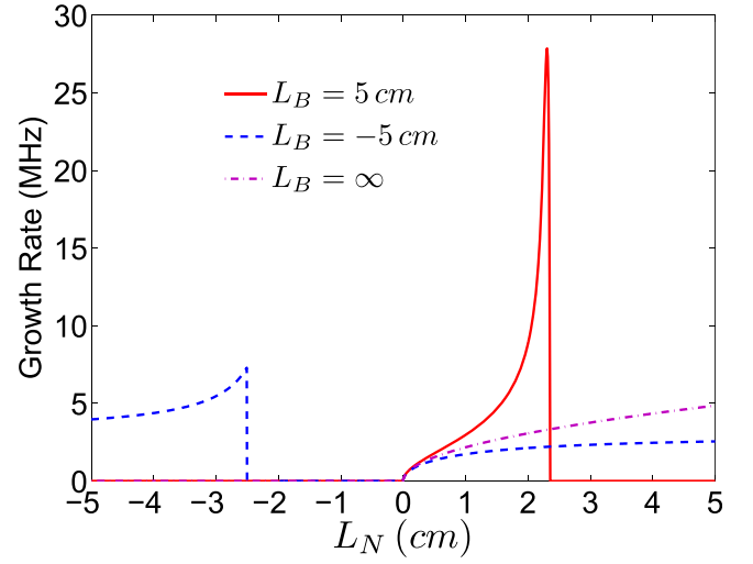
FIG. 5. Growth rate as a function of L_N for different values of L_B when L_T is 1 cm.
