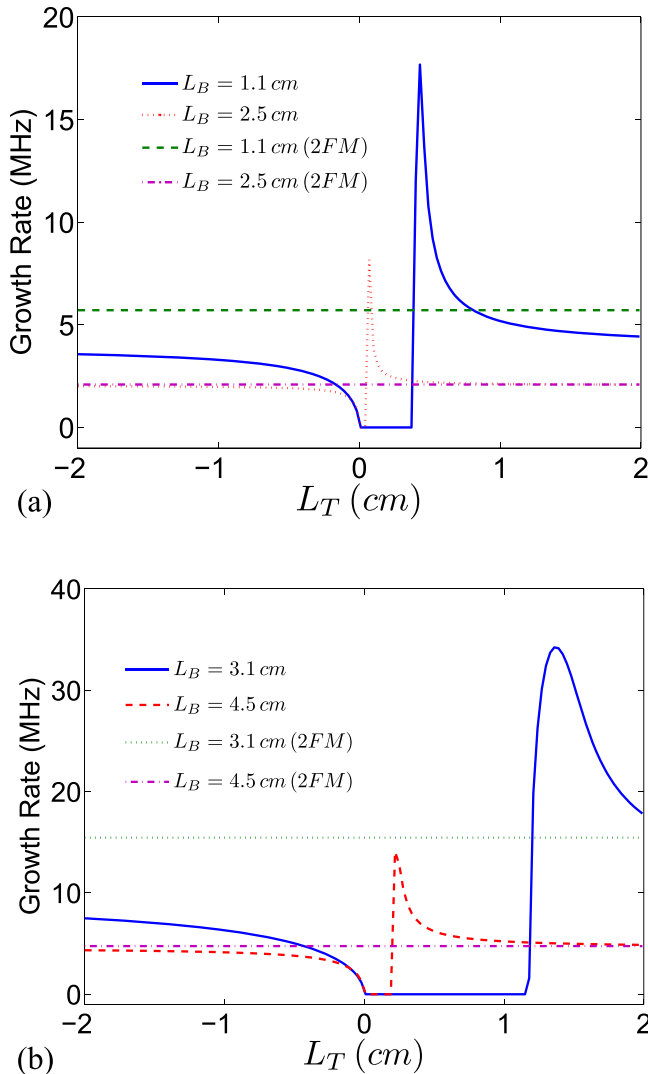
FIG. 7. Growth rate as a function of L_T for (a) L_N = 0.5 cm and (b) L_N = 1.5 cm, for different values of L_B . The straight lines correspond to the values predicted by the two-field model.
