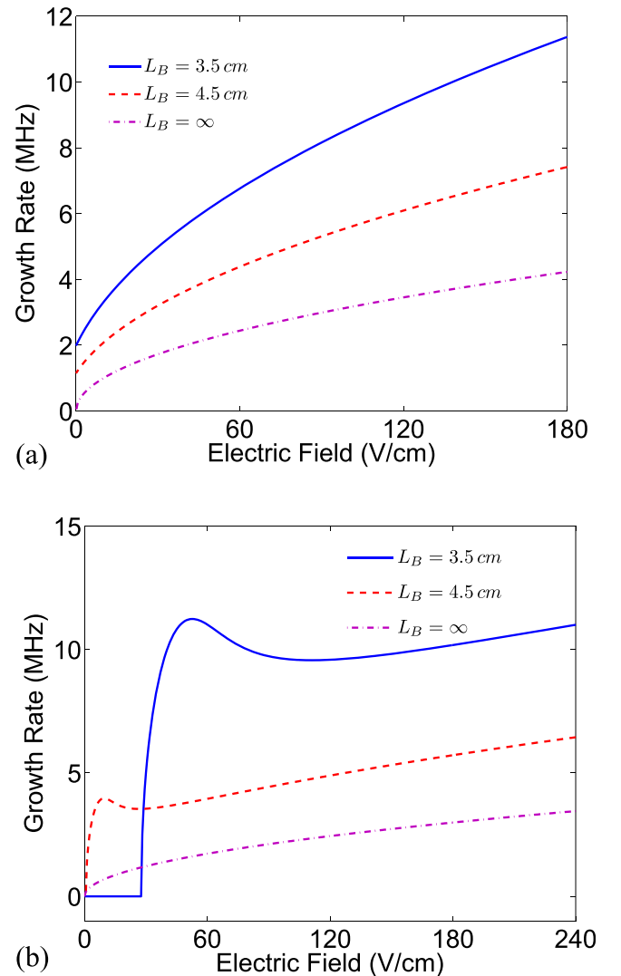
FIG. 8. Growth rate as a function of the electric field for L_N = 1.5 cm as predicted by (a) the two-field model and (b) the three-field model, L_T = 1 cm.
